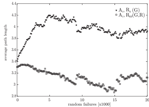
(b) Robustness of graphs resulting from A_1 in a random failure scenario
